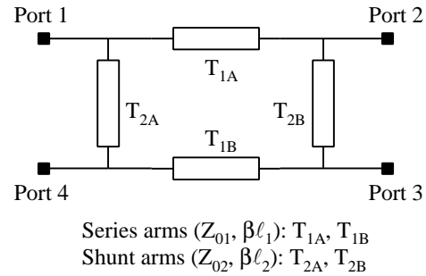
Fig.1 The branch-line quadrature hybrid.
