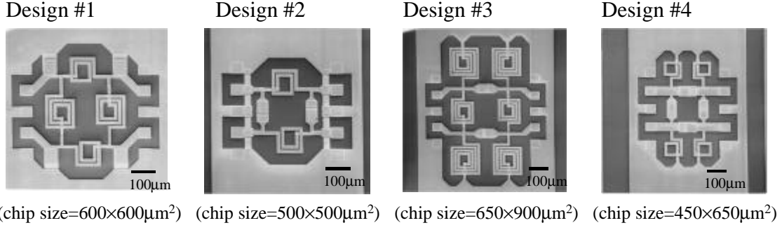
Fig. 3 The photomicrograph of the lumped quadrature designs.
