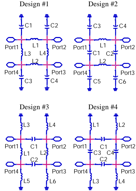
Fig. 2 The schematic of the lumped quadrature hybrids.
